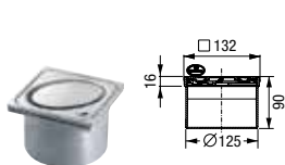
1 nasadka z ABS, Rama □ 132 mm
