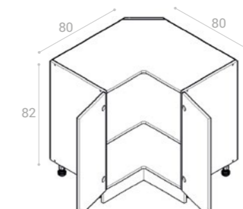
SN/90/90
