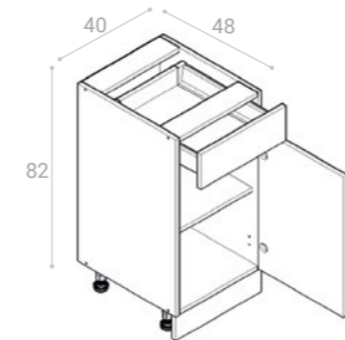
S/40/1 MODERNBOX
