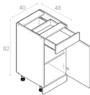
S/40/1
