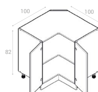
SN/100/100
