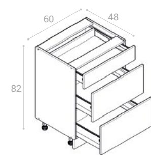
S/60/3 METALBOX
