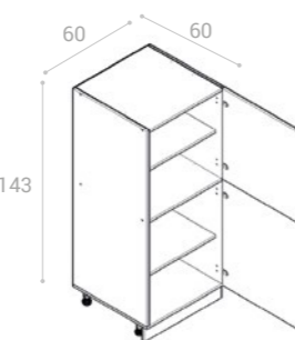
S/60/143
