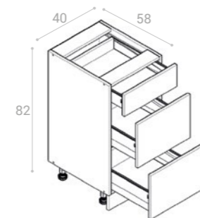
S/40/3 MODERNBOX
