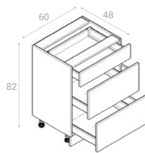
S/60/3 MODERNBOX
