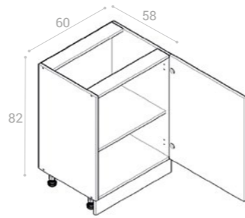
S/60
