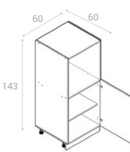
SP/60/143
