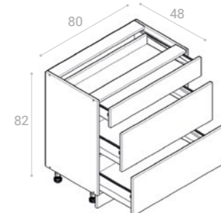
S/80/3 METALBOX
