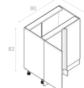
SN/100
