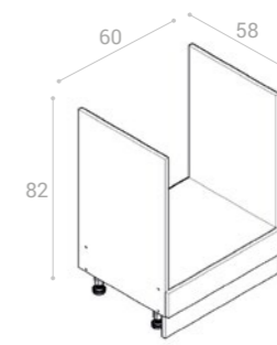
SP/60
