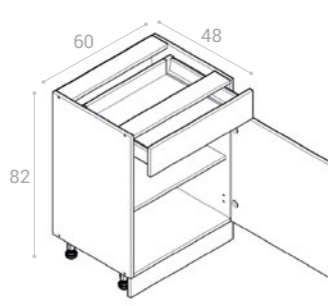
S/60/1 MODERNBOX
