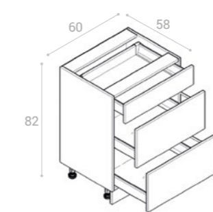
S/60/3 MODERNBOX
