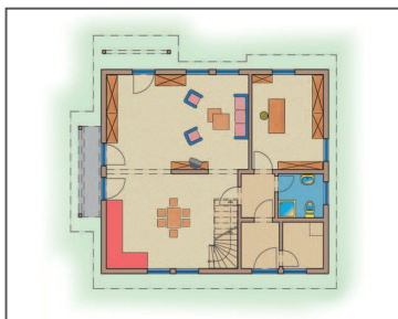
parter 77 m 2
